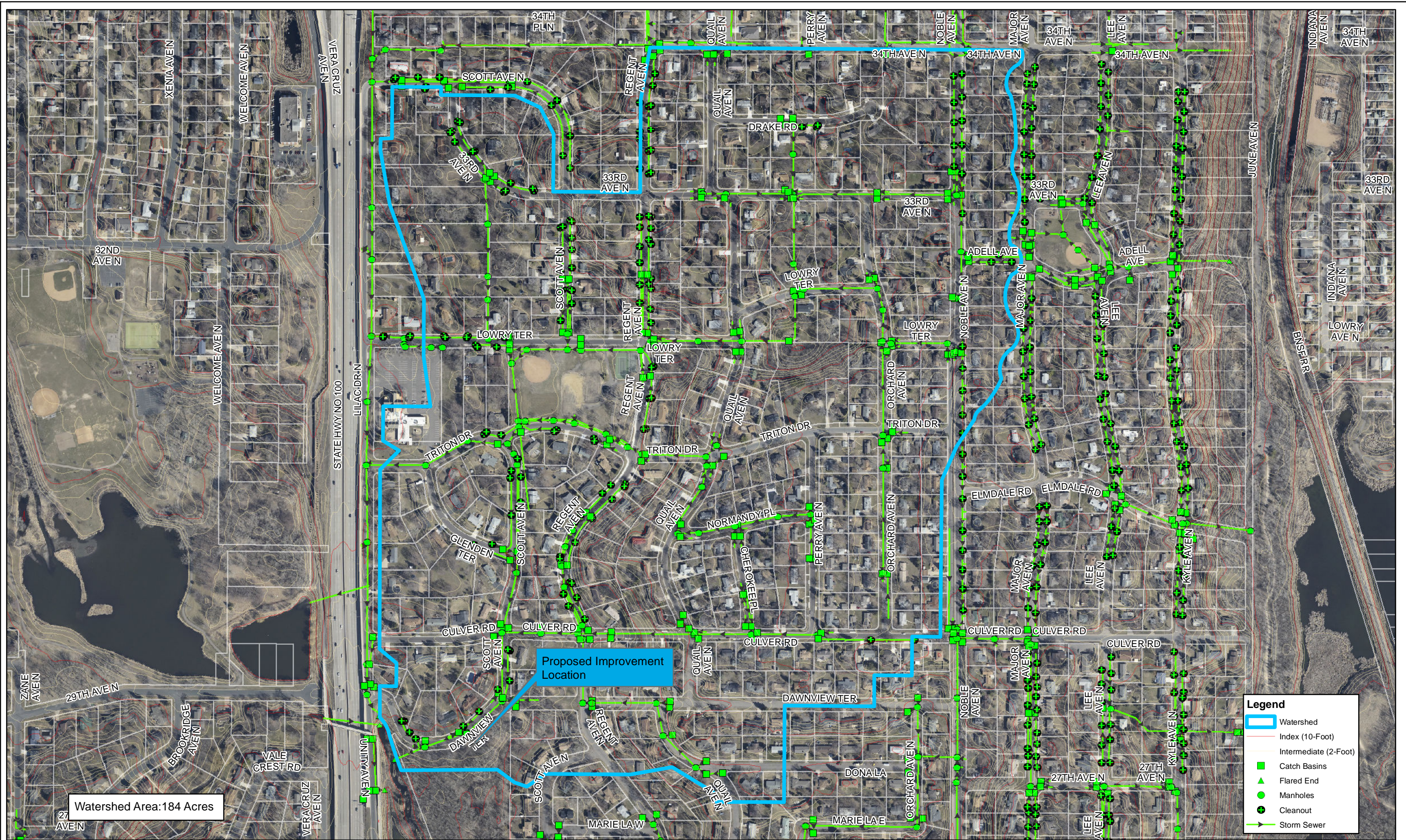
Briarwood/Dawnview Water Quality Improvement Project Watershed, Storm Sewer, & Topography City of Golden Valley, MN
