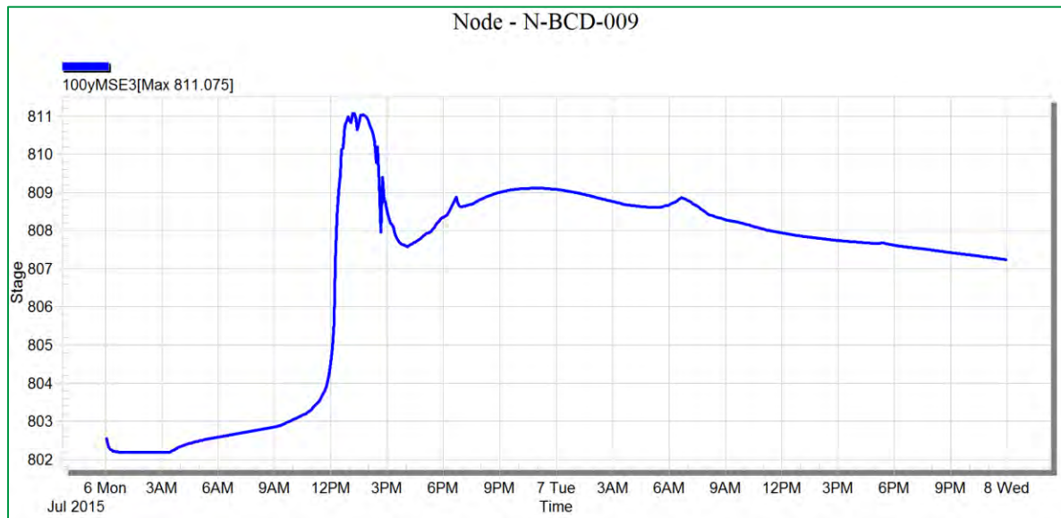
Figure 1: Base Scenario (Existing Conditions) Hydrograph
