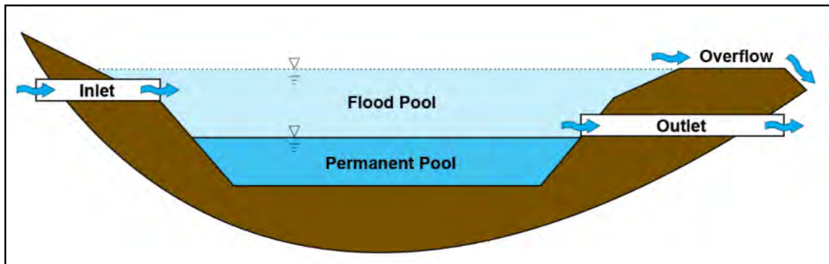
Figure 3-2 Typical storm water pond configuration
