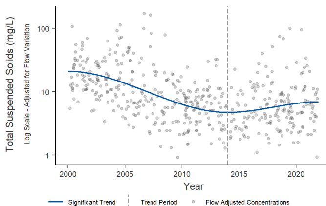
Figure 1: Statistical Trend Graph for Total Suspended Solids
